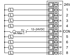
Single Power Source
