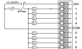
Dual Power Source
